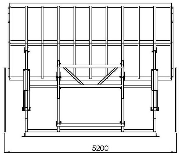
POSITION DEVERSEMENT
